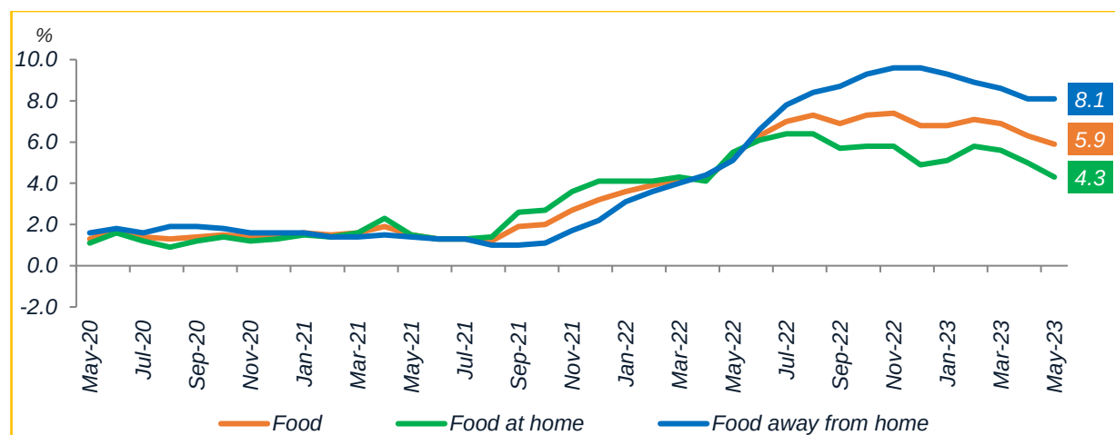
Chart 7 Inflation for Food & Non-Alcoholic Beverages, May 2020 – May 2023
