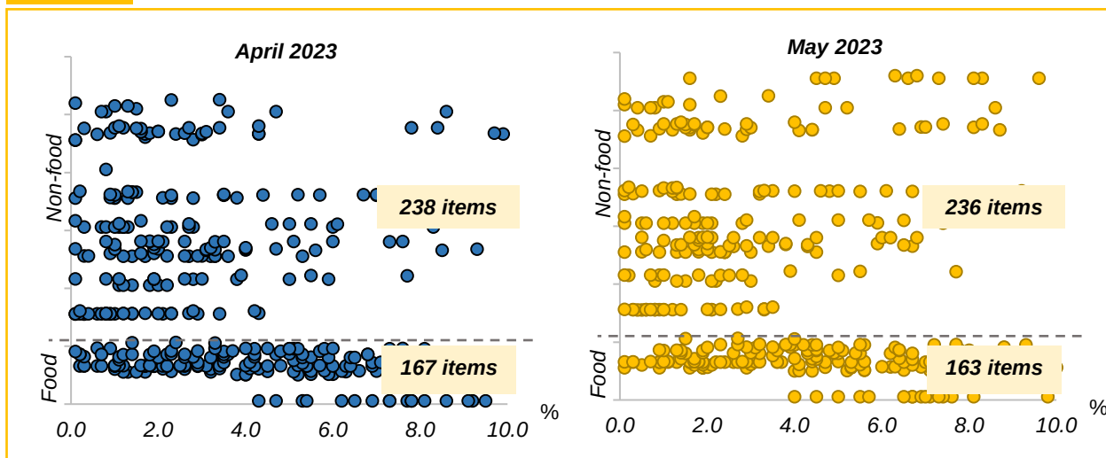
Chart 6 Distribution of Inflation for Food and Non-Food that Increased ≤10%, April 2023 & May 2023
