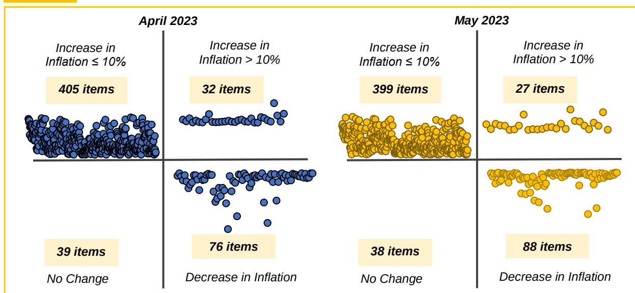
Chart 5 Inflation by Quadrant, April 2023 & May 2023
