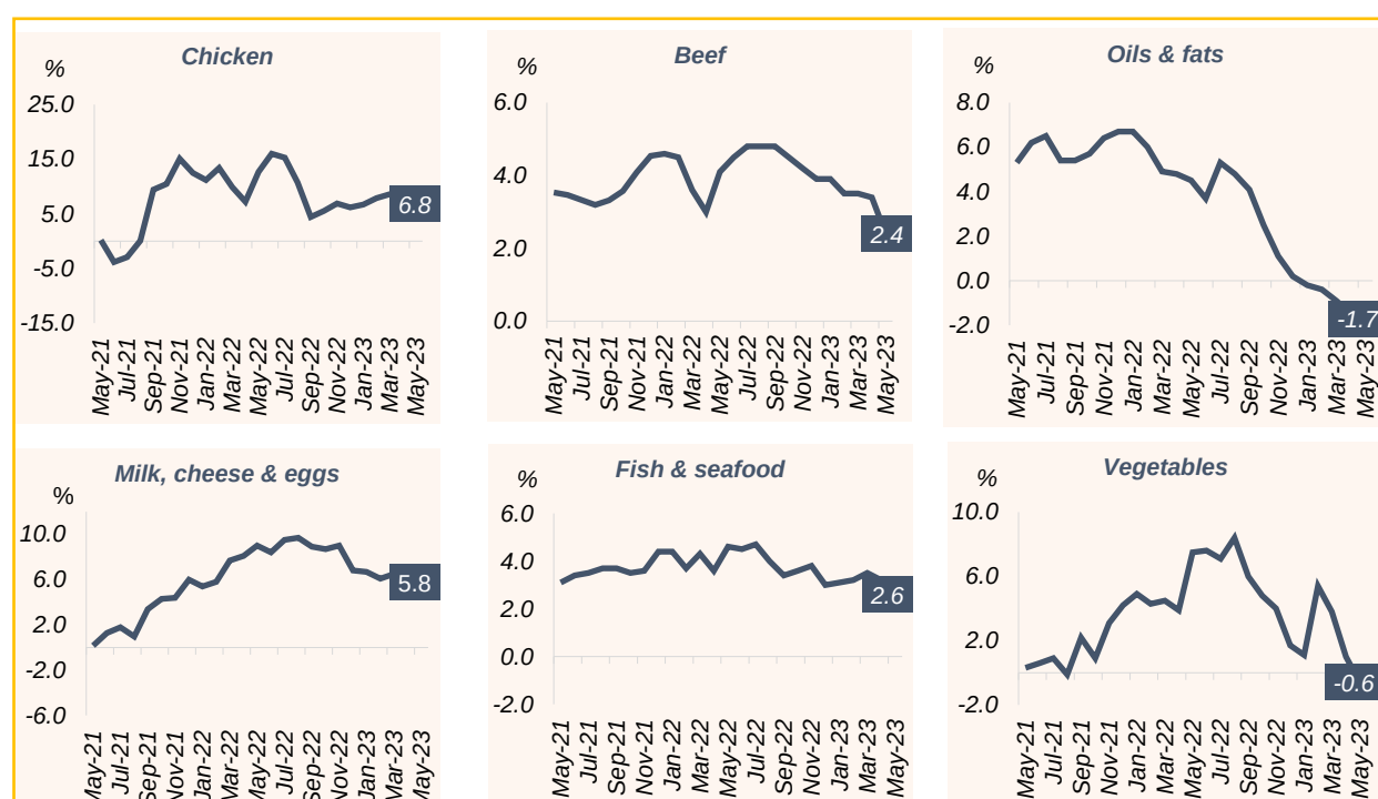
Chart 11 Selected Food Inflation for Income Group Below RM3,000, May 2021 – May 2023
