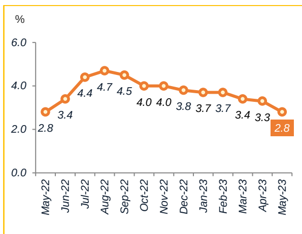
Chart 1 Malaysia Headline Inflation, May 2022 – May 2023
