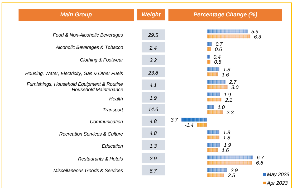
Chart 3 Inflation by Main Group, April 2023 & May 2023
