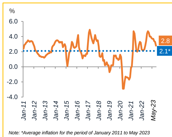
Chart 2 Malaysia Headline Inflation, January 2011 – May 2023
