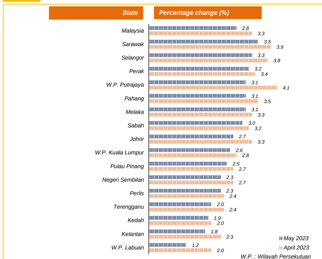
Chart 8 Inflation by State, April 2023 & May 2023
