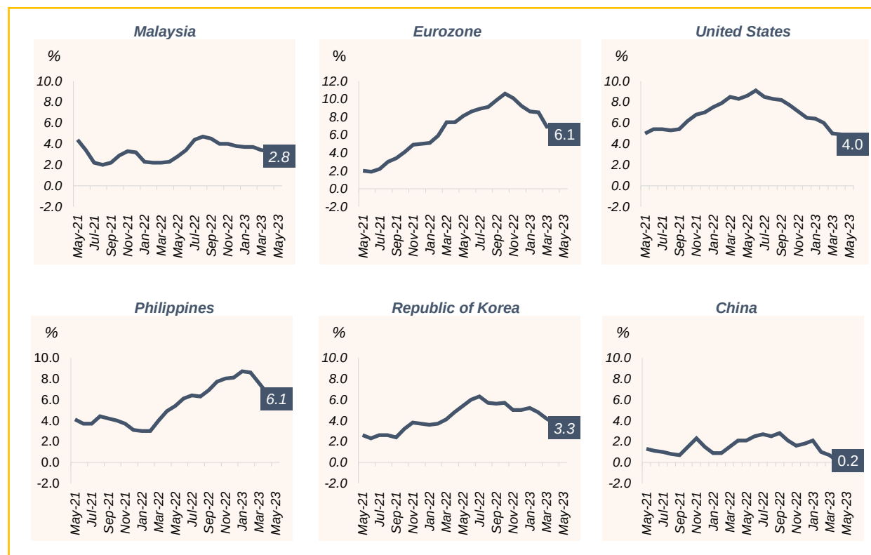
Chart 12 Inflation for Selected Countries, May 2021 – May 2023
