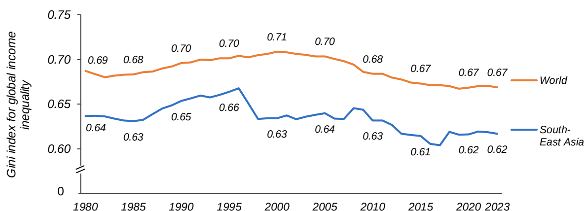
Chart 7 Global Gini Index, 1980 - 2023
