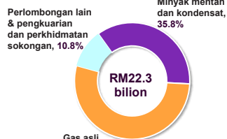
Gas asli, 53.4%
